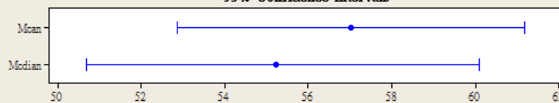
95% Confidence Intervals
